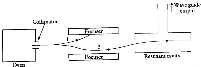
14.8 The ammonia maser. Molecules produced by the oven are collimated, selected into the upper level 2 by the inhomogeneous focusing field, and then passed through the maser cavity. The whole apparatus is placed in an evacuated vessel.
